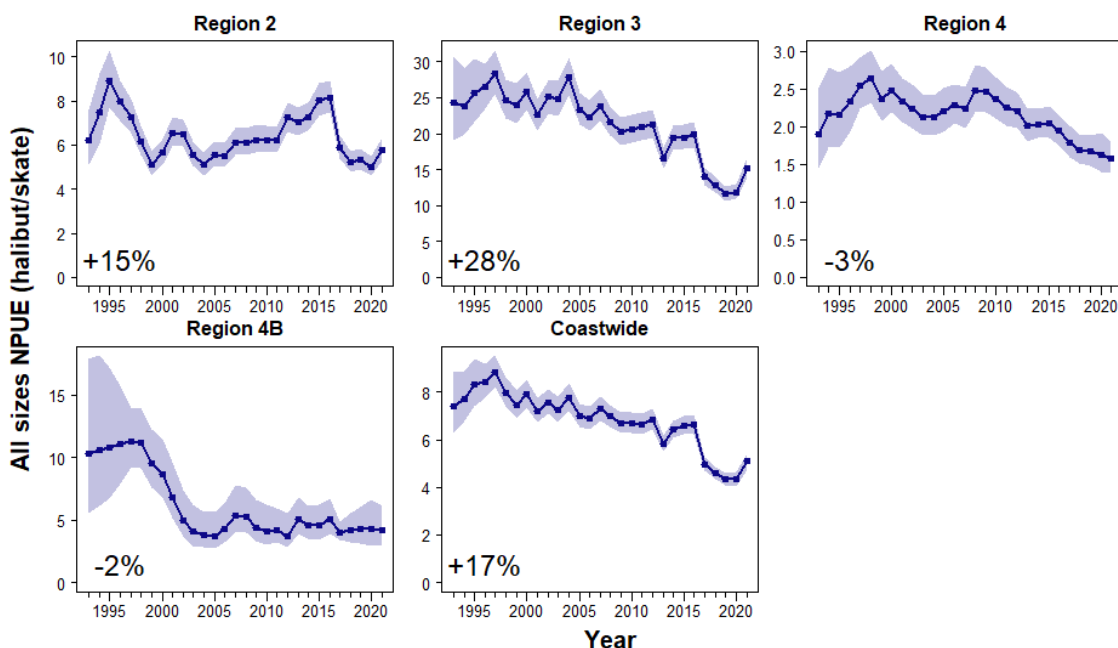
FIGURE 2. Trends in modeled survey NPUE by Biological Region, 1993-2021. Percentages indicate the change from 2020 to 2021. Shaded zones indicate 95% credible intervals.
