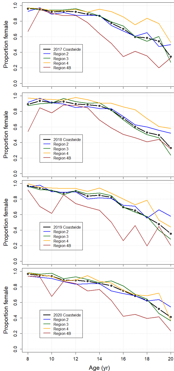
FIGURE 38. Estimates of the sex-ratio-at-age of the commercial fishery landings by Biological Region from 2017 to 2020 (upper to lower panels).
