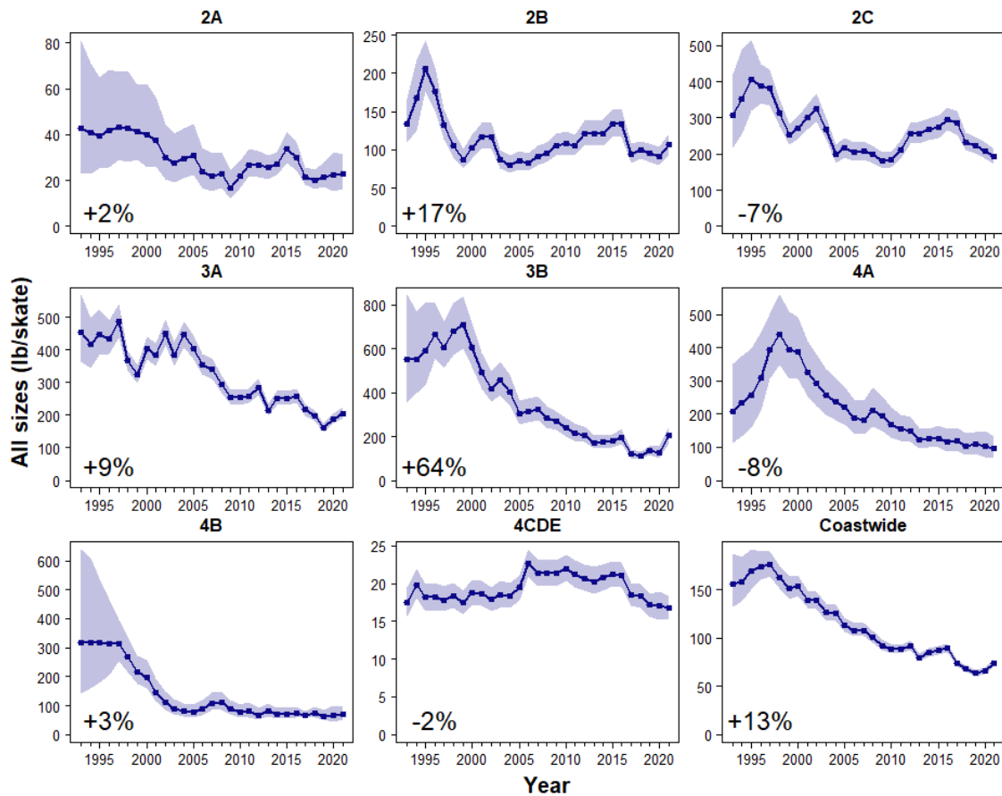
FIGURE 5. Trends in survey WPUE estimated from the space-time modelling by IPHC Regulatory Area, 1993-2021. Percentages indicate the estimated change from 2020 to 2021. Shaded zones indicate 95% credible intervals.
