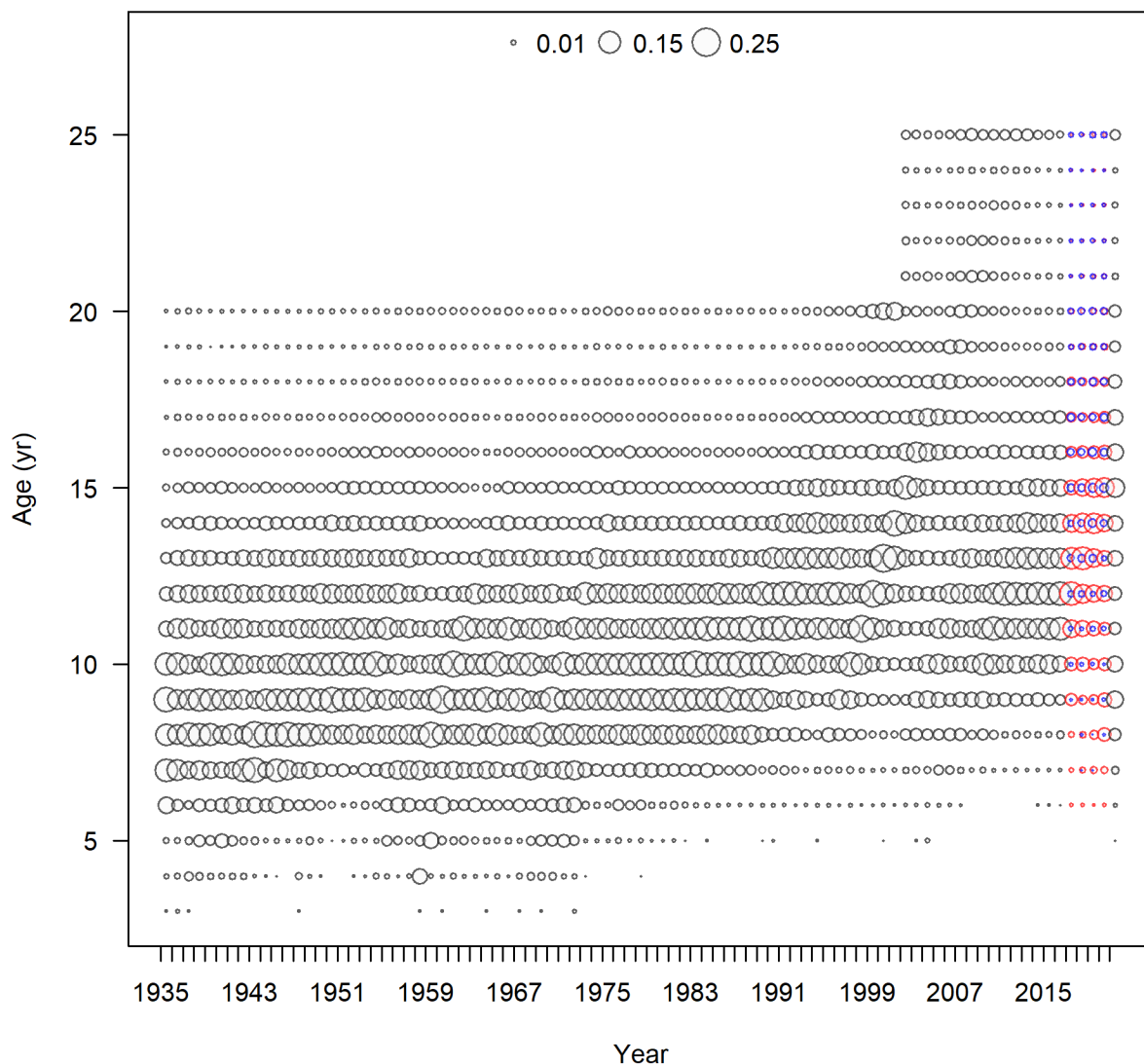
FIGURE 40. Historical coastwide commercial fishery proportions-at-age from the retained catch. Note that the current 32 inch (82.3 cm) minimum size limit was implemented in 1973. Circles sum to 1.0 within each year (column). For 2017-2020, males are delineated by blue circles and females by red circles at each age.
