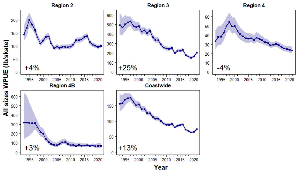
FIGURE 4. Trends in survey WPUE estimated from the space-time modelling by Biological Region, 1993-2021. Percentages indicate the estimated change from 2020 to 2021. Shaded zones indicate 95% credible intervals.
