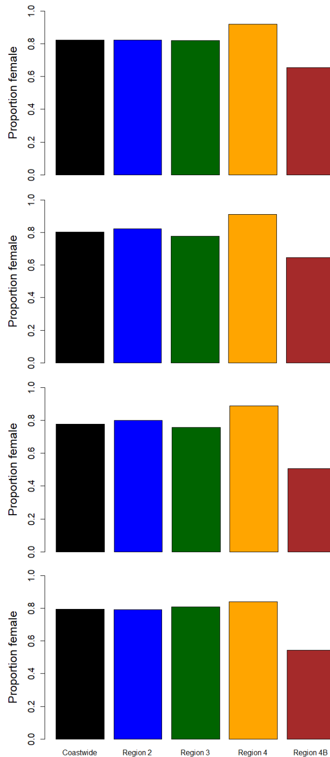
FIGURE 37. Estimates of the sex ratio of the commercial fishery landings by Biological Region from 2017 to 2020 (upper to lower panels).
