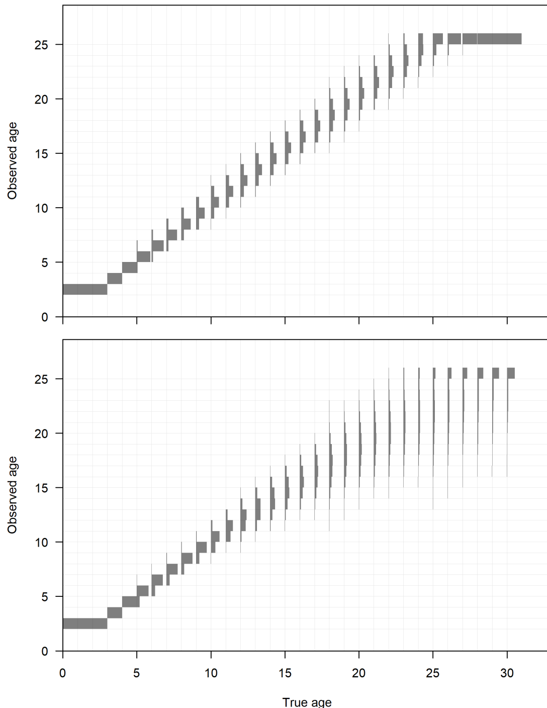
FIGURE 51. Ageing bias and imprecision relationships used in recent stock assessments
