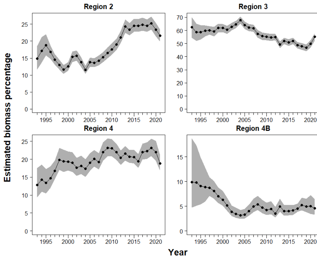
FIGURE 8. Estimated biological stock distribution (1993-2021) calculated from model output of survey WPUE of all sizes of Pacific halibut captured by the FISS. Shaded zones indicate 95% credible intervals.
