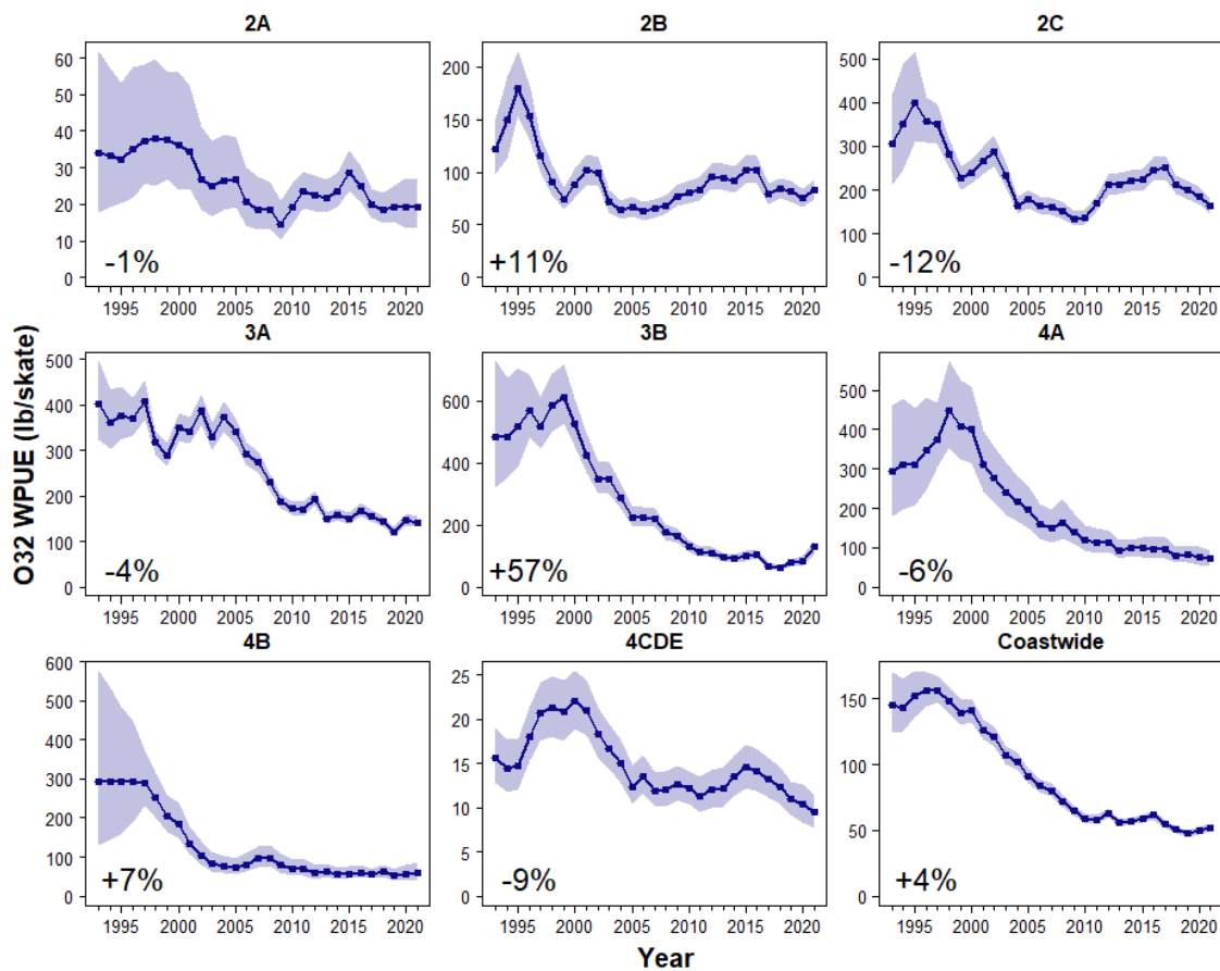
FIGURE 7. Trends in survey legal (O32) WPUE estimated from the space-time modelling by IPHC Regulatory Area, 1993-2021. Percentages indicate the estimated change from 2020 to 2021. Shaded zones indicate 95% credible intervals.
