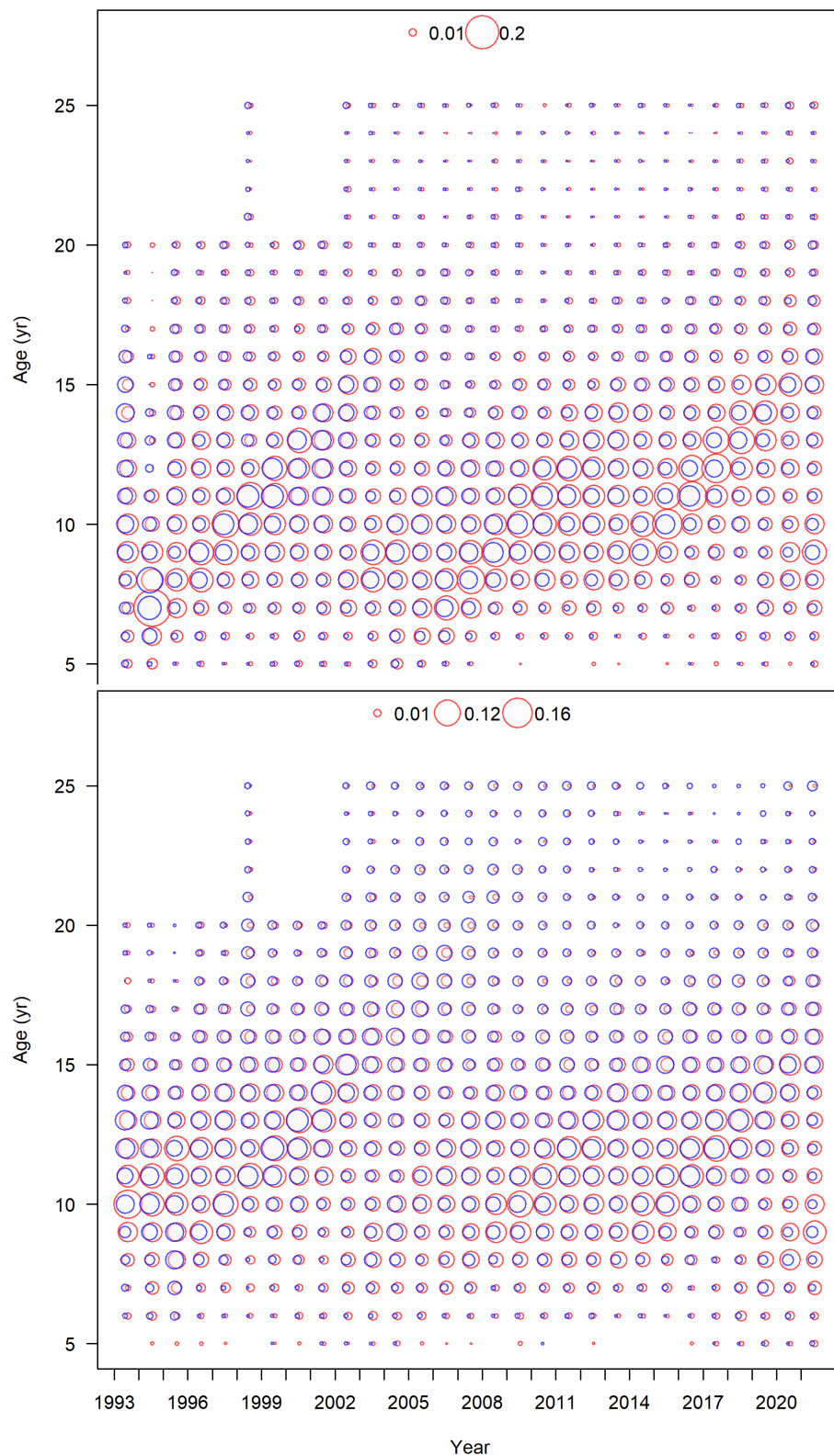
FIGURE 11. Recent proportions-at-age for female (red circles) and male (blue circles) Pacific halibut captured by the FISS from Biological Region 2 (upper panel) and Region 3 (lower panel). Proportions sum to 1.0 across both sexes within each year.
