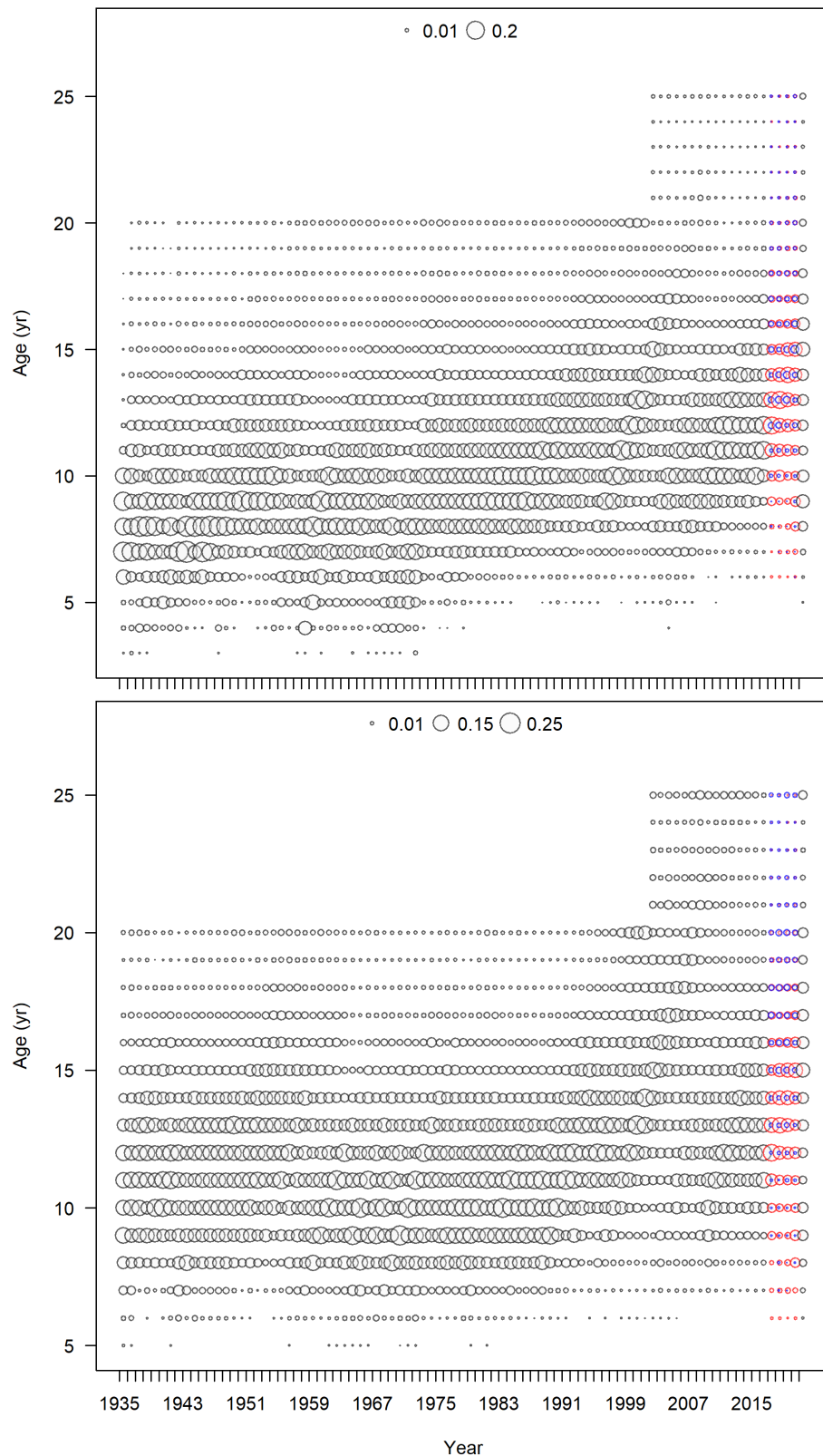
FIGURE 41. Commercial fishery proportions-at-age in the retained catch (male and female Pacific halibut combined) for Biological Region 2 (top panel), and Region 3 (bottom panel). Circles sum to 1.0 within each year (column). For 2017-2020, males are delineated by blue circles and females by red circles at each age.
