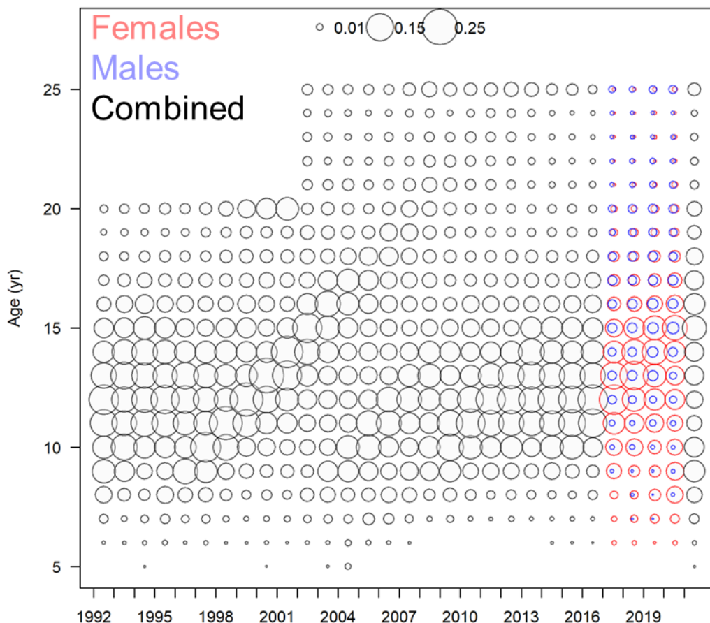
FIGURE 39. Estimates of recent commercial fishery proportions-at-age. Circles sum to 1.0 within each year (column). For 2017-2020, males are delineated by blue circles and females by red circles at each age.
