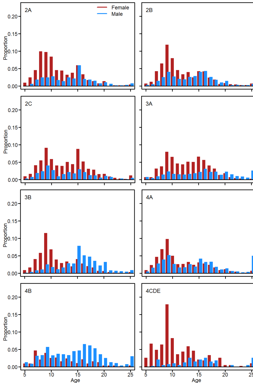
FIGURE 9. Age distributions from the 2021 FISS by IPHC Regulatory Area. Red bars indicate the proportion of females (by number) in the FISS catch, and the blue bars indicate proportions for male Pacific halibut.
