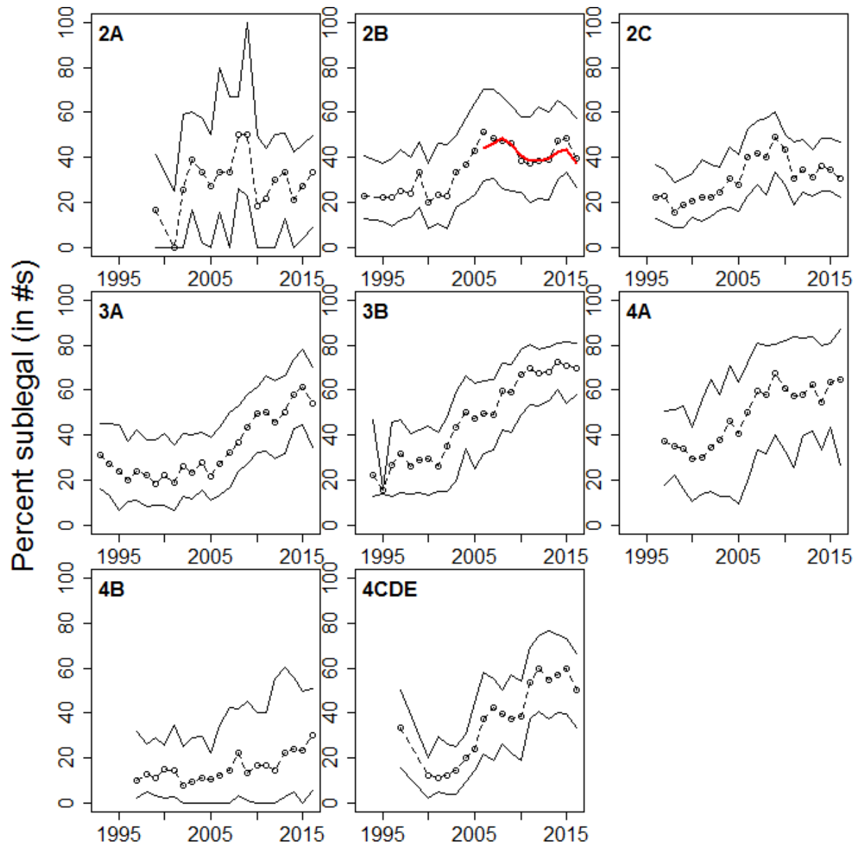
FIGURE B10. Trends in percent sublegal (<32'') halibut catch by the setline survey 1993-2016 (From: Goen et al. 2017b). Circles denote median survey station percent sublegal; lines denote the 25 th and 75 th percentiles. Solid line in Area 2B denotes the percent sublegal reported in directed commercial Pacific halibut fishery logbooks
