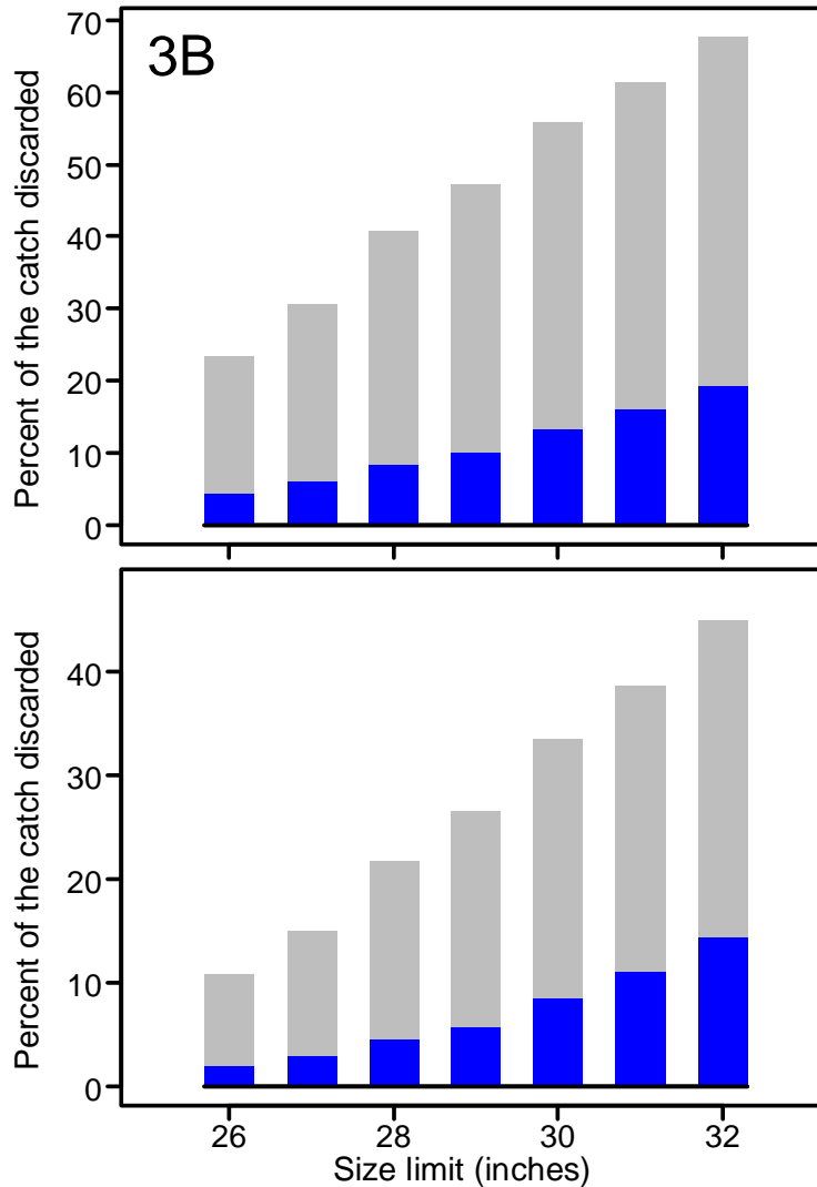
FIGURE B5. Percentage of the 2016 survey catch discarded in Area 3B for size-limits from 26 to 32 inches, based on the number of fish (upper panel) and the weight of fish (lower panel). Height of the bars represents the total, and the darker (lower) portion the contribution of male halibut. Note that the y-axes differ. See tables for percentage values.
